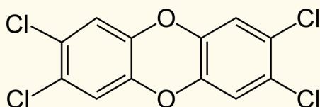
Dioxin
